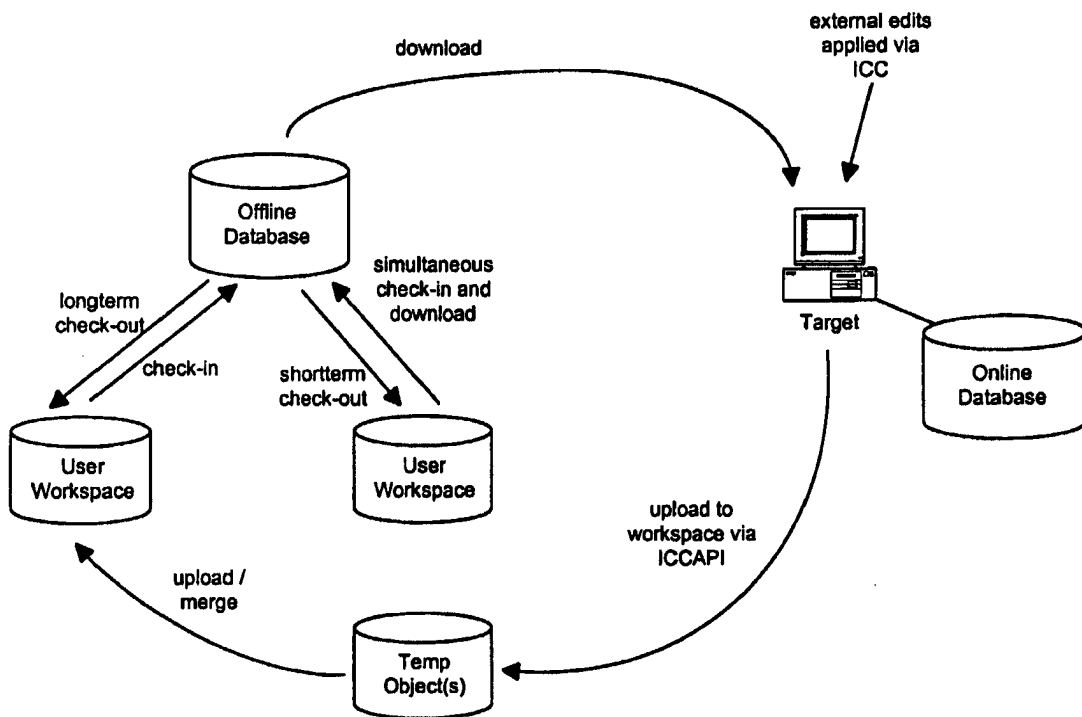
Figure 45 - Version Control - Basic Concepts
